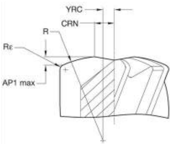
FH200-H schematic diagram of 6 flute endmill shaeer blade
